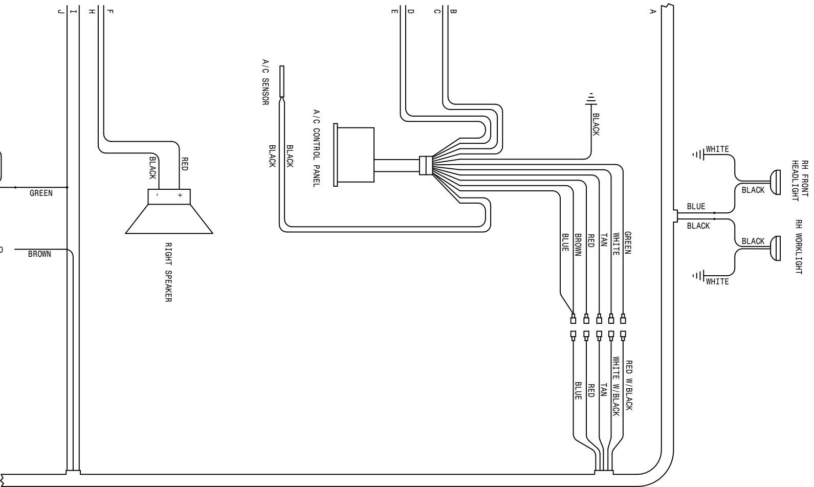
293266 - CAB WIRE HARNESS
