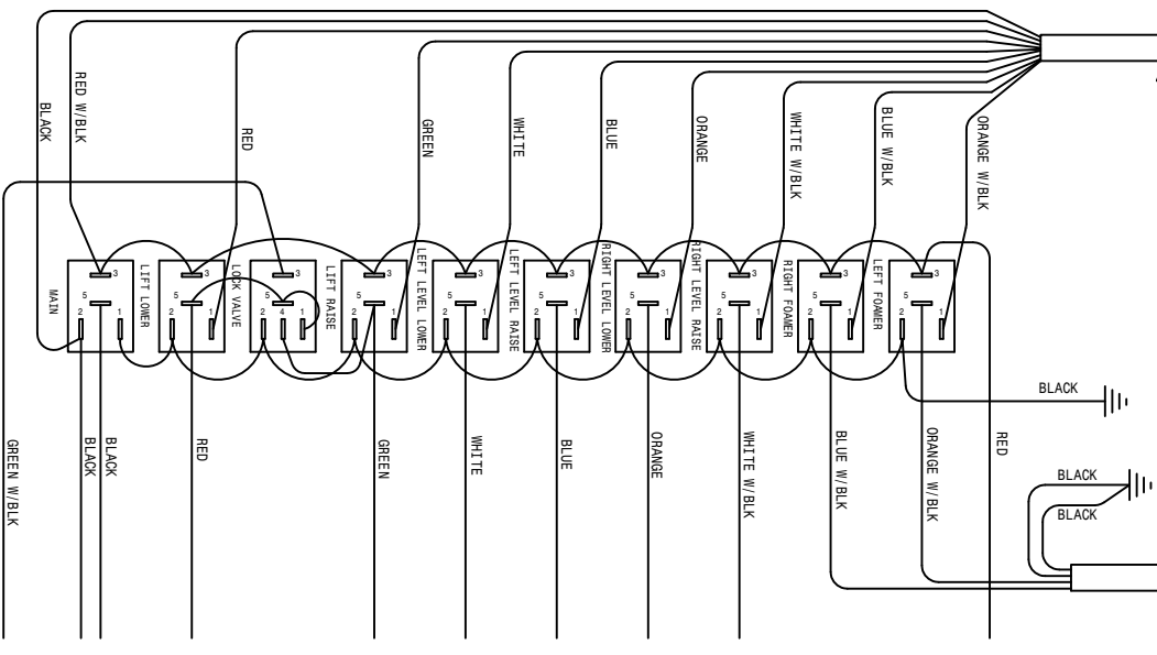
293733 - FOAM HARNESS CONSOLE 2101 03
