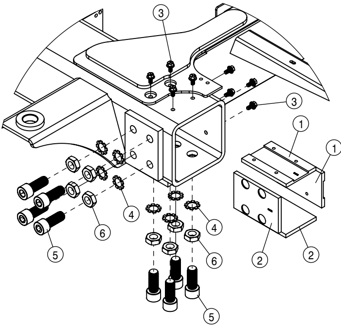
FRONT MAINFRAME
